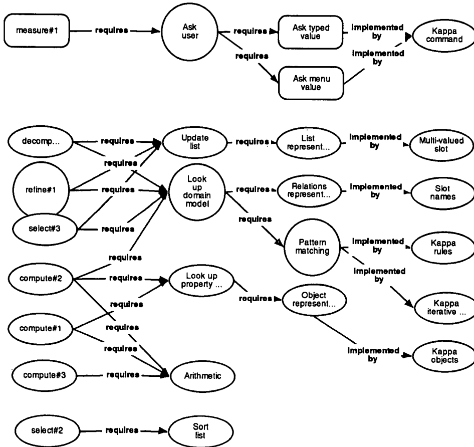
Figure 8 Design model: diagnosing faults in machinery
