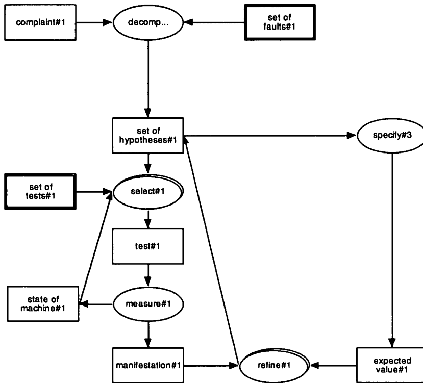
Figure 6 Inference structure: machine fault diagnosis
