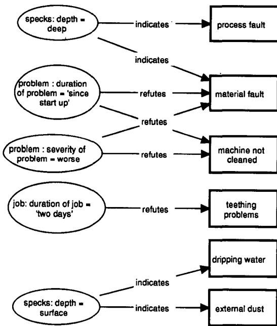
Figure 5 A domain model which links expressions with concepts
