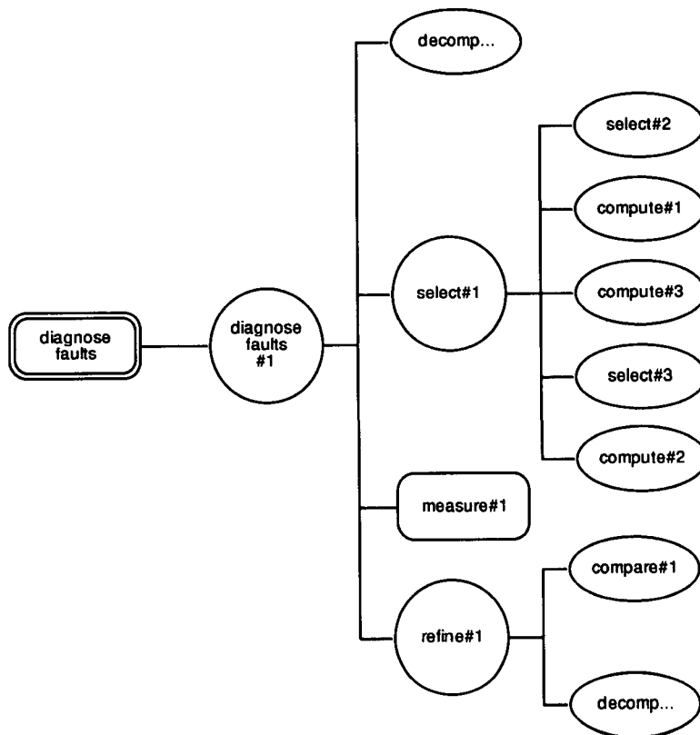
Figure 7 Task structure: machine fault diagnosis
