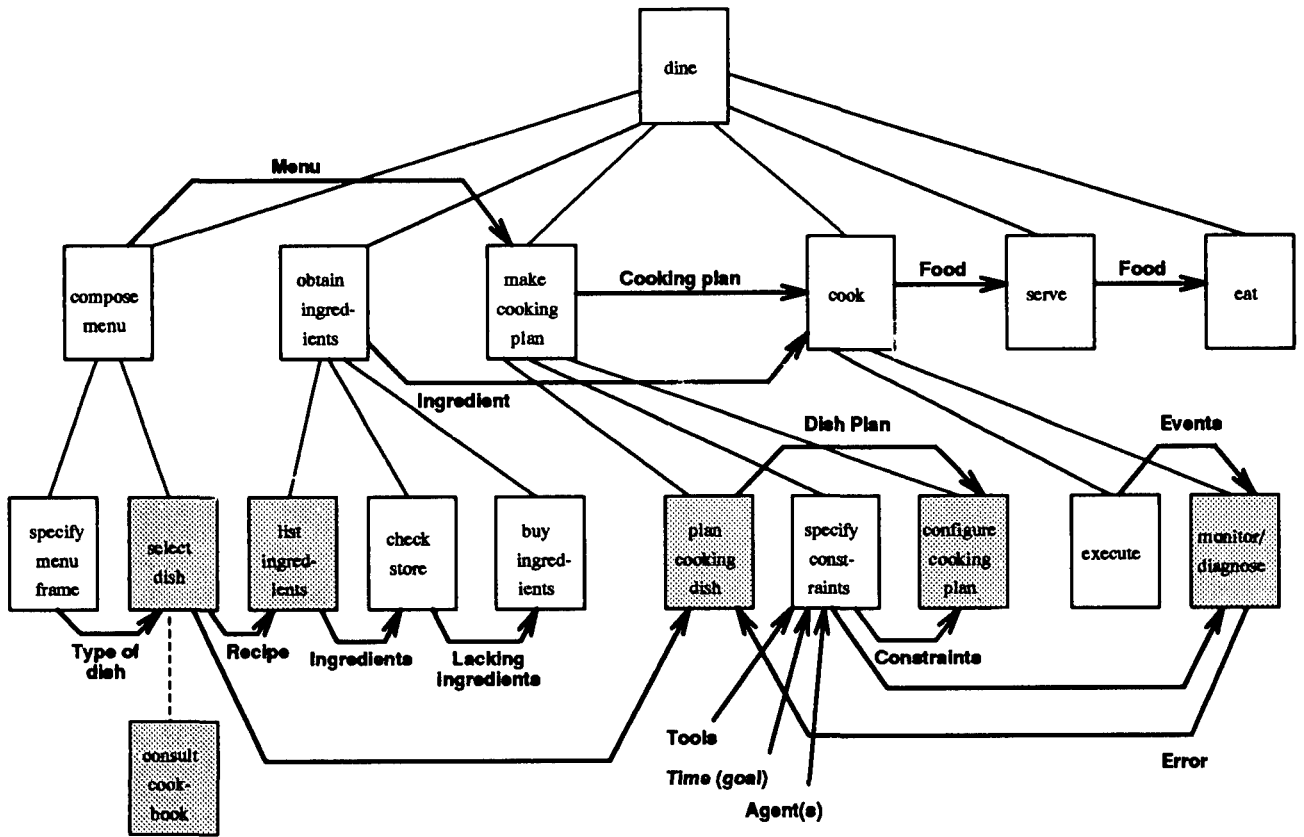
Figure 2 Task model: preparing a meal
