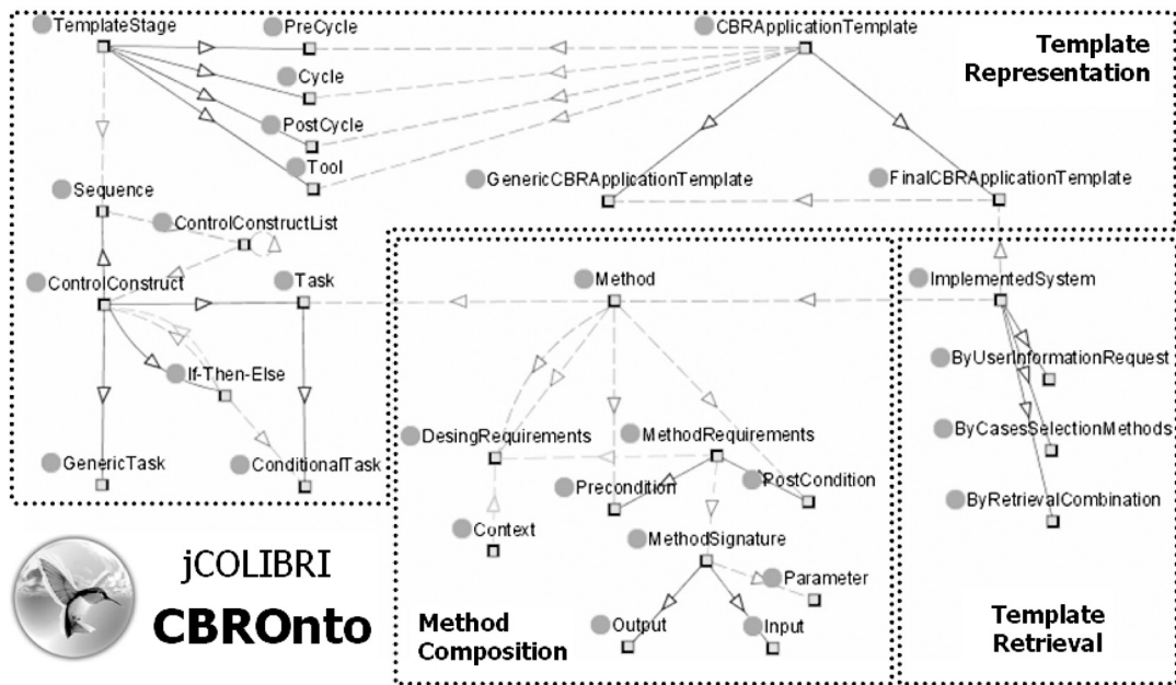
Figure 3 CBROnto overview
