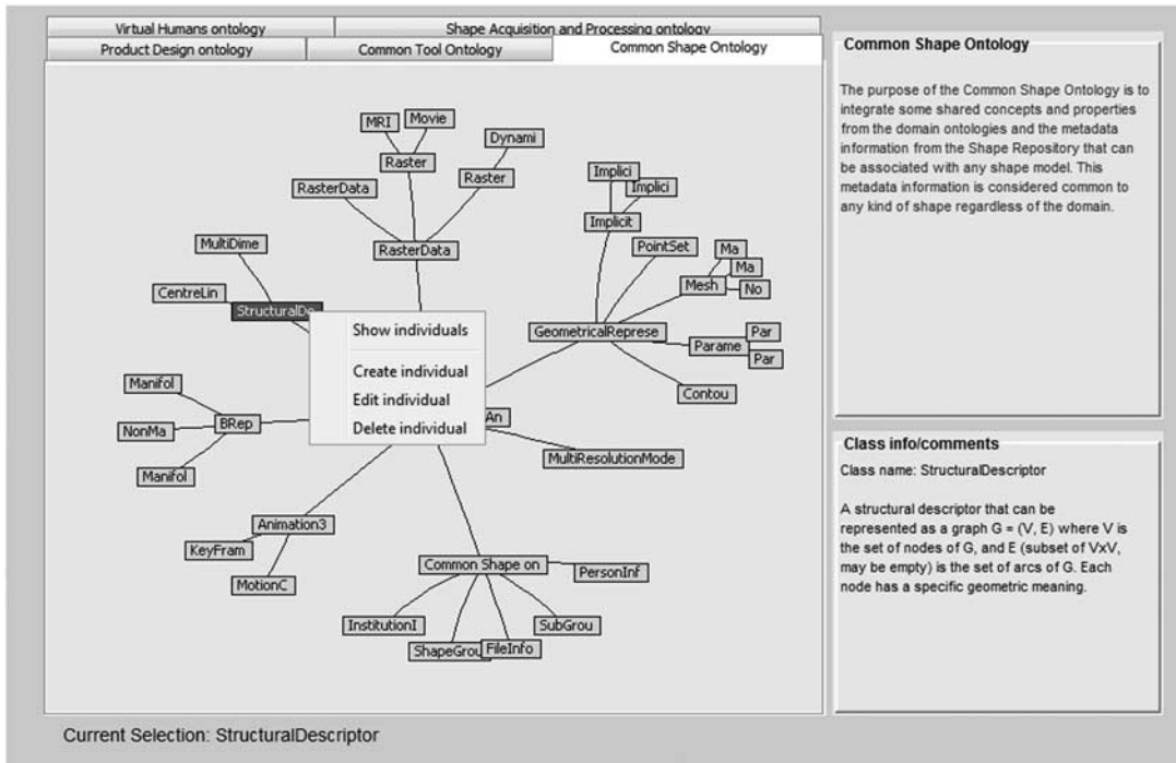
Figure 7 The hyperbolic tree visualization tool
