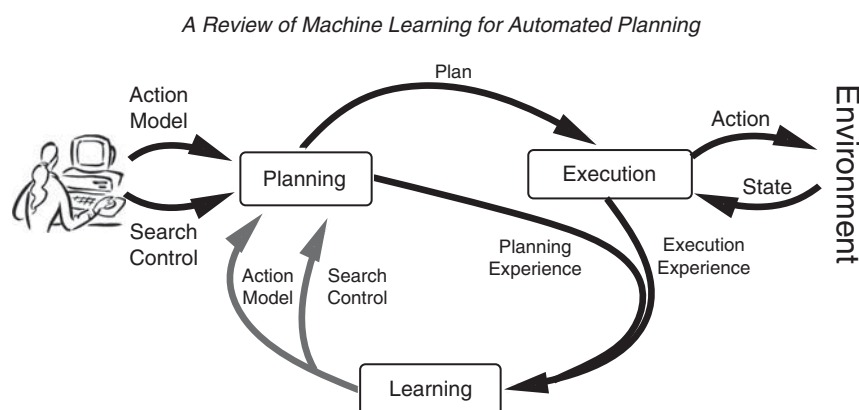
Figure 1 Use of Machine Learning to improve the knowledge of the Automated Planning processes
