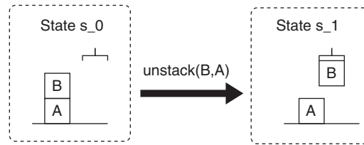
Figure 3 Example of application of the unstack action in a fully observable and deterministic Blocksworld
