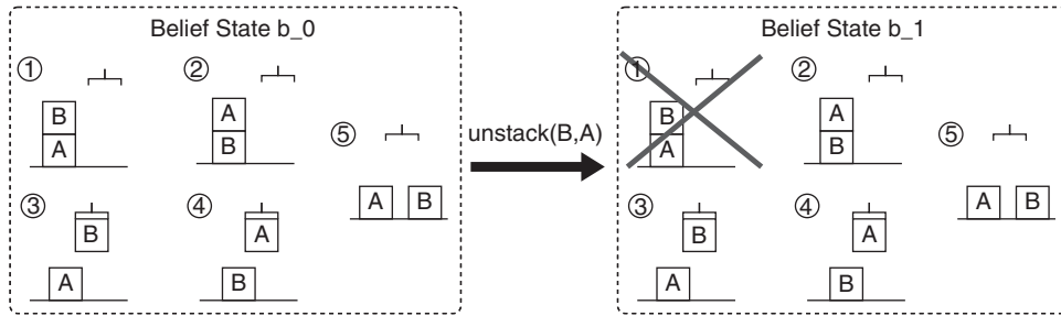
Figure 5 Example of application of the unstack(B, A) action in a non-observable two-blocks Blocksworld
