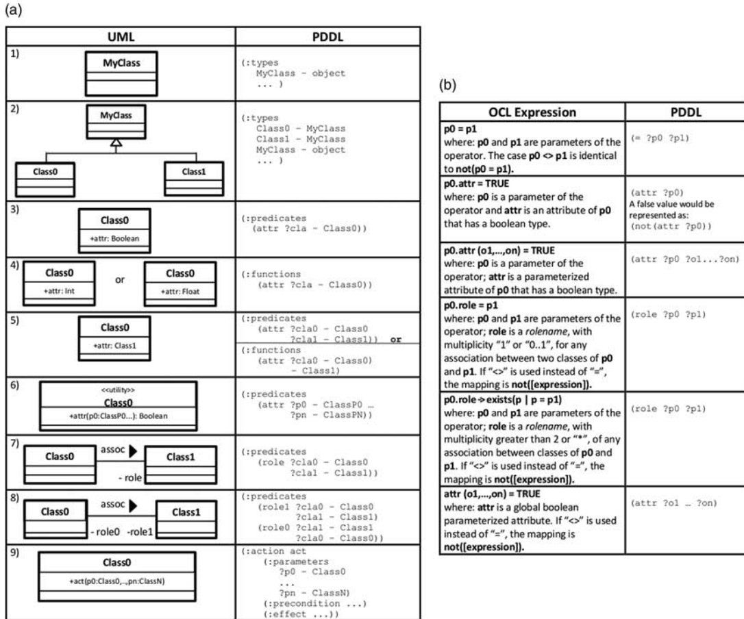
Figure 3 (a) Mapping PDDL types, predicates and functions from UML class diagrams; (b) Mapping OCL expression to PDDL conditions. PDDL = Planning Domain Definition Language; UML = Unified Modeling Language; OCL = Object Constraint Language
