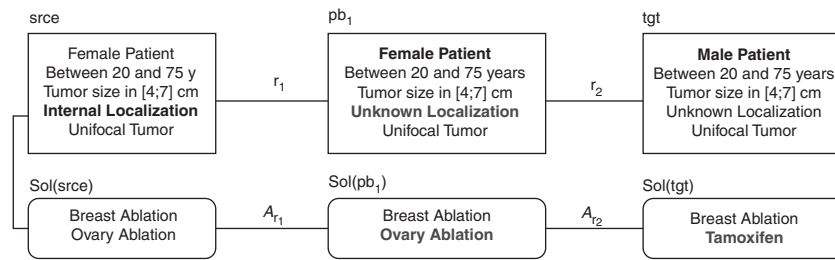
Figure 4 An example of CBR problem-solving using reformulations, with similarity path from srce to tgt on first line and corresponding adaptation path from Sol(srce) to Sol(tgt) on the second line. CBR = case-based reasoning
