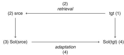
Figure 2 The case-based inference. (1) A target problem is provided to the CBR system. (2) The system retrieves a source problem similar to the target problem. (3) The source problem is a problem associated with a solution. (4) The system adapts this solution in order to solve the target problem
