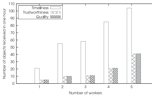
Figure 5 Source selection using different QoC-based conflict resolving policies. QoC = Quality of Context
