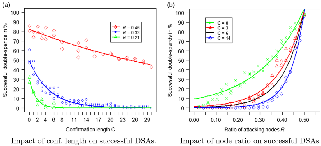
Figure 6 Successful DSAs for different numbers of confirmation blocks
