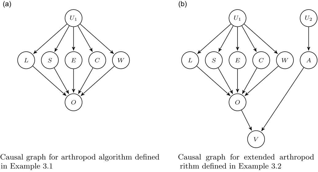
Figure 1 (a) Causal graph for arthropod algorithm defined in Example 3.1 (b) Causal graph for extended arthropod algorithm defined in Example 3.2.
