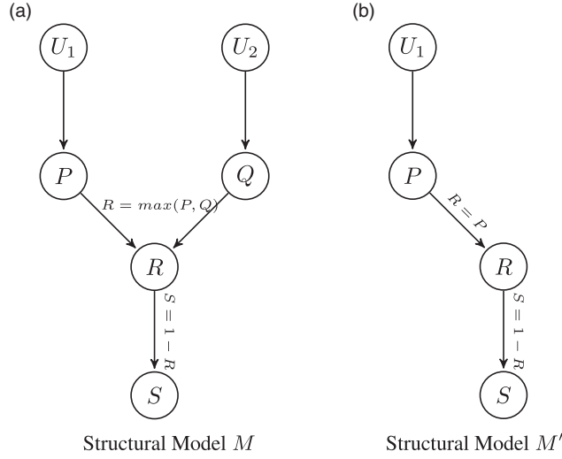
Figure 2 Structural Models for Example 5.6.
