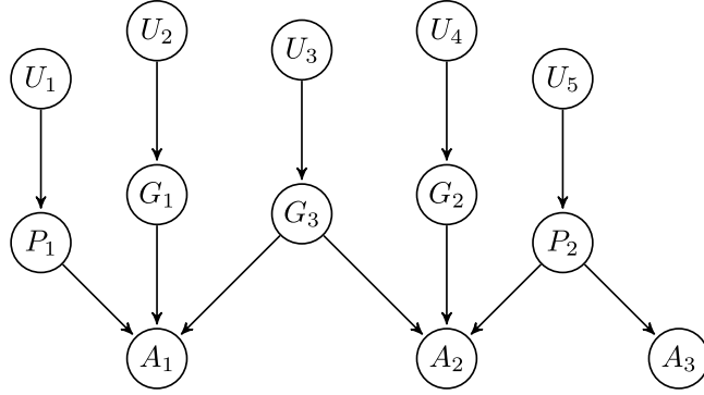
Figure 3 Causal graph for goal-directed planning.
