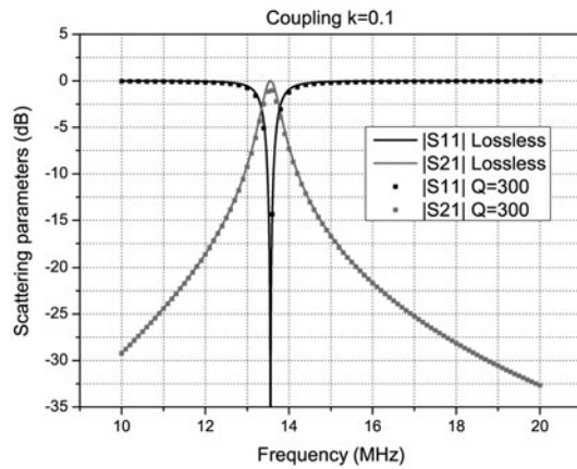
Fig. 13. A 1:1 transformer, operating at the frequency of 13.56, has been designed by using an immittance inverter with the Tee( L , C , L ) configuration. In the graph are reported the responses in the lossless case and in the case of resonators with Q = 300 . The coupling coefficient is also shown in the legend. With reference to Fig. 12, the component values are: L_1 = L_2 = 1 \mu\text{H} , C_1 = C_2 = 137.8 \text{ pF} . For the figure on the left, we have M = 0.3 \mu\text{H} , C_3 = 459 \text{ pF} , whereas for the figure on the right we have selected M = 0.1 \mu\text{H} and C_3 = 1.378 \text{ nF} .
