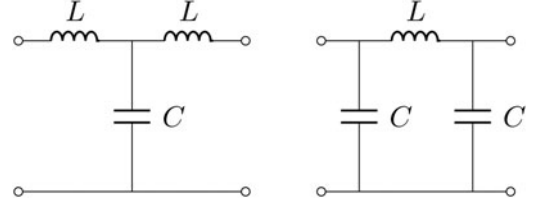
Fig. 7. LC immittance inverters: the Tee( L, C, L ) representation is shown on the left side and provides an inverter value of \omega_0 L , when equation (7) is satisfied. On the right side is shown a Pi network with values Pi(C, L, C) , which realizes an immittance inverter of value \omega_0 L .
