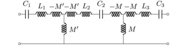
Fig. 14. A 1:1 transformer realized with two wireless immittance inverters. At a selected frequency \omega = \omega_0 , the series of L_1 , C_1 , L_2 , C_2 , and L_3 , C_3 realize short circuits and the entire network behaves as two immittance inverters. When M' is adjusted to be equal to M , a 1:1 wireless transformer is realized.
