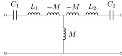
Fig. 9. Coupled inductances equivalent network with added capacitances C_1 and C_2 . At a selected frequency \omega = \omega_0 , the series of L_1 , C_1 and L_2 , C_2 realize a short circuit and the entire network behaves as an impedance inverter.
