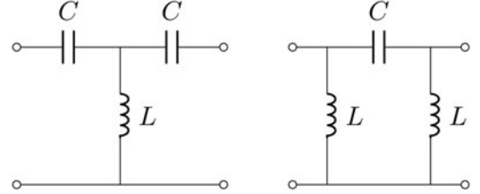
Fig. 8. LC immittance inverters: the Tee( C, L, C ) representation is shown on the left side and provides an inverter value of -\omega_0 L , when equation (7) is satisfied. On the right side is shown a Pi network with values Pi(L, C, L) which realizes an immittance inverter of value -\omega_0 L .
