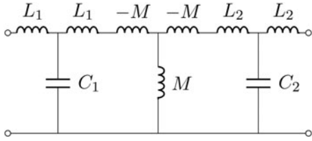
Fig. 11. A parallel capacitance C_1 and a parallel capacitance C_2 have been added respectively on ports 1 and 2. Further addition at ports 1 and 2 of the series inductors L_1 , L_2 , results in the structure shown in the figure. Note that at port 1 the Tee( L_1 , C_1 , L_1 ) represents another impedance inverter. Thus, at a selected frequency \omega = \omega_0 , the entire network behaves as three cascaded immittance inverters.
