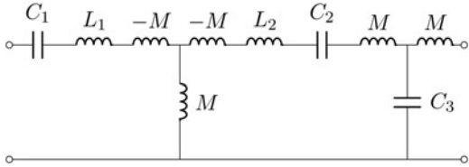
Fig. 12. A 1:1 transformer realized with one wireless immittance inverter and one lumped inverter. At a selected frequency \omega = \omega_0 , the series of L_1 , C_1 and L_2 , C_2 realize a short circuit and the entire network behaves as two immittance inverters.
