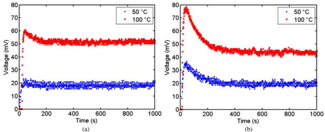
Fig. 5. Voltage generated by the TEG versus time at two different heat-gun temperatures: (a) stand-alone TEG; (b) antenna-TEG system.
