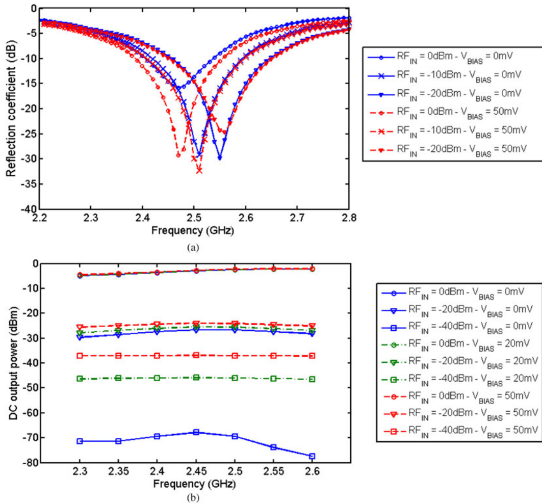
Fig. 7. Measured reflection coefficient (a) and output power (b) versus frequency and assuming the input RF power and the polarization voltage as variable parameters.
