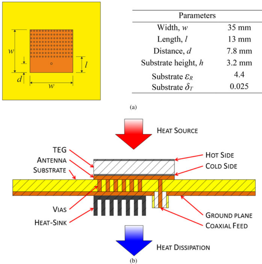
Fig. 1. Top view of the antenna layout and its dimensions (a) (© 2014 IEEE. Reprinted, with permission, from [18]) and section of the antenna-TEG structure with thermal flux (b).
