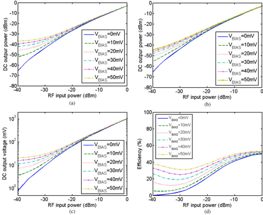
Fig. 8. Rectifier measurements: (a) overall dc output power, P_{DC\_OUT} (see equation (1)); (b) output power related to the RF-to-dc conversion only, P_{DC\_OUT\_R2D} (see equation (2)); (c) dc output voltage; (d) efficiency (see equation (3)). The measurements are functions of the RF input power at 2.45 GHz.
