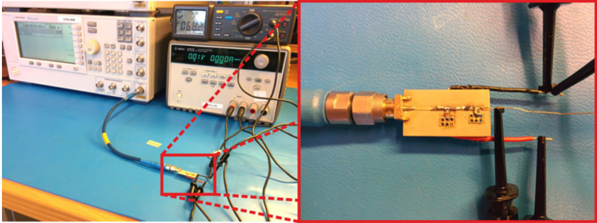
Fig. 6. Measurement setup with zoom on the DUT.
