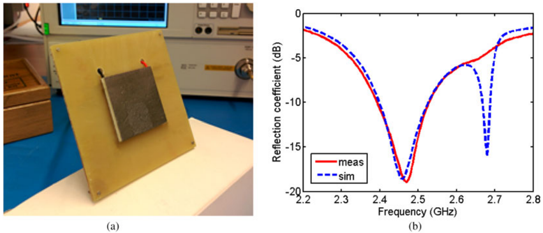
Fig. 3. Prototype of the antenna with TEG (a) and reflection coefficients (b). Prototype of the antenna with TEG (a) (© 2014 IEEE. Reprinted, with permission, from [18]) and reflection coefficients (b).
