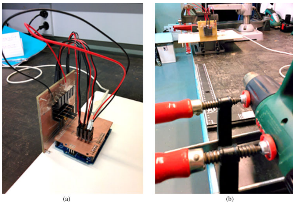
Fig. 4. Assembled antenna-TEG prototype with acquisitions system (a) and measurement setup (b).
