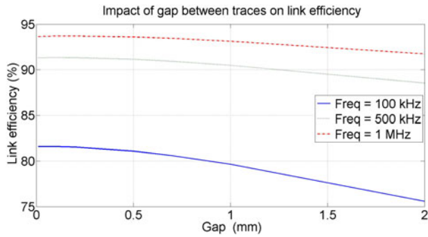
Fig. 10. Link efficiency as function of the gap between traces (number of turns n = 10 turns, trace width w = 0.85 mm, copper thickness t = 35 \mu\text{m} , and inner radius IR = 10.5 mm).
