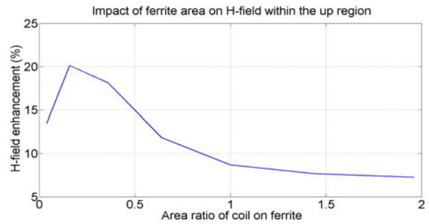
Fig. 26. H -field enhancement as function of the ratio of areas of coil and ferrite (other parameters frozen to their standard value).
