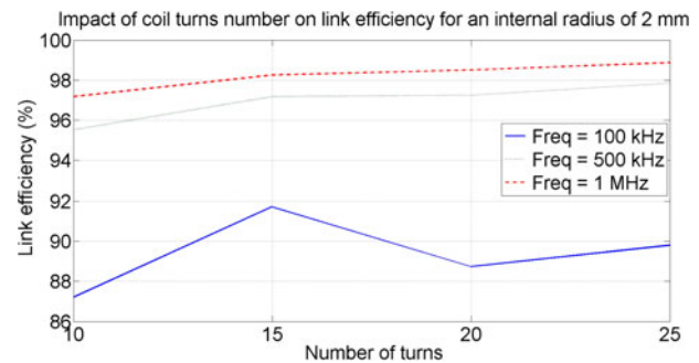
Fig. 13. Link efficiency as function of turns number for IR = 2 mm ( t = 70 \mu\text{m} , g = 0.1 mm, and w = 0.85 mm).
