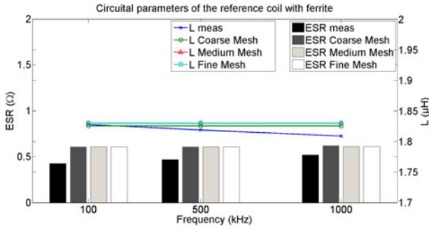
Fig. 19. Impact of the different modeling approaches adopted for simulations of the RFC1 coil with a ferrite square positioned below.
