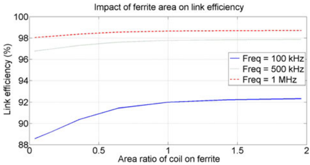
Fig. 24. Link efficiency as function of the ratio of areas of coil and ferrite (other parameters frozen to their standard value).
