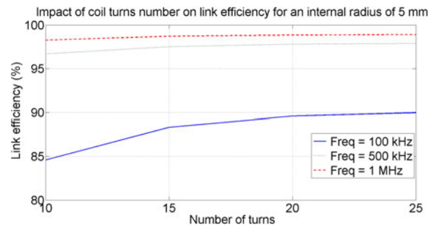
Fig. 14. Link efficiency as function of turns number for IR = 5 mm ( t = 70 \mu\text{m} , g = 0.1 mm, and w = 0.85 mm).
