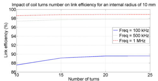
Fig. 15. Link efficiency as function of turns number for IR = 10 mm ( t = 70 \mu\text{m} , g = 0.1 mm, and w = 0.85 mm).
