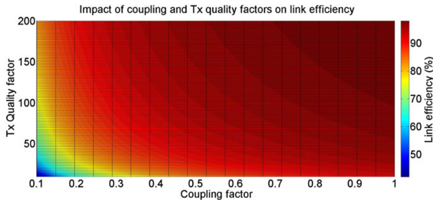
Fig. 2. Link efficiency formula in function of Tx quality factor and coupling factor ( Q_{Rx} = 15 ).
