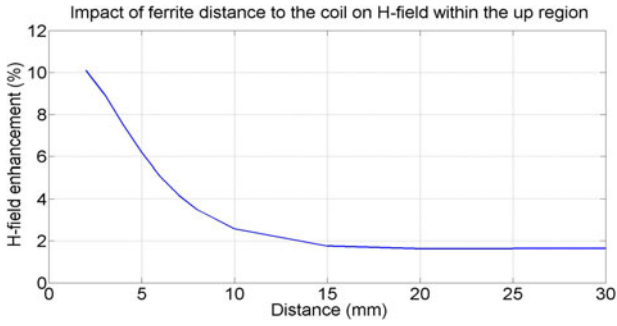
Fig. 23. H -field enhancement as function of the distance between coil and ferrite (other parameters frozen to their standard value).
