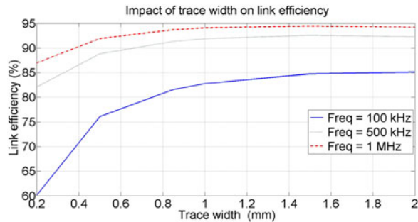
Fig. 12. Link efficiency as function of trace width ( n = 10 turns, t = 35 \mu\text{m} , g = 0.1 mm, inner radius, and IR = 10.5 mm).
