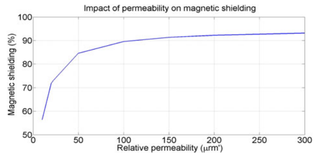
Fig. 28. Magnetic shielding as function of the magnetic permeability of the ferrite (other parameters frozen to their standard value).
