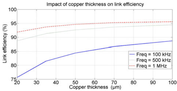
Fig. 11. Link efficiency as function of copper thickness ( n = 10 turns, w = 0.85 mm, g = 0.1 mm, and inner radius IR = 10.5 mm).
