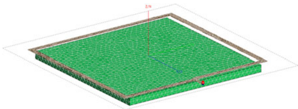
Fig. 17. Modeled reference coil with ferrite.
