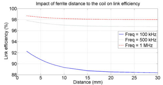
Fig. 21. Link efficiency as function of the distance between Tx coil and the ferrite (other parameters frozen to their standard value).
