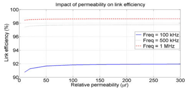
Fig. 27. Link efficiency as function of the magnetic permeability of the ferrite (other parameters frozen to their standard value).
