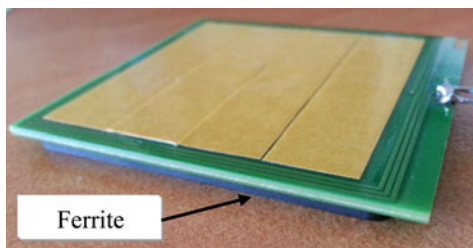
Fig. 18. Prototyped reference coil (RFC1) with the ferrite positioned below (left: top view, right: bottom view).
