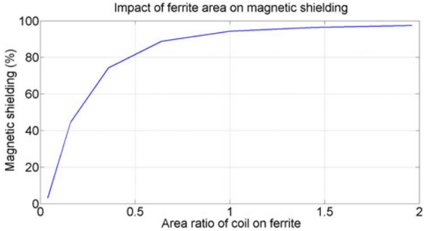
Fig. 25. Magnetic shielding as function of the ratio of areas of coil and ferrite (other parameters frozen to their standard value).
