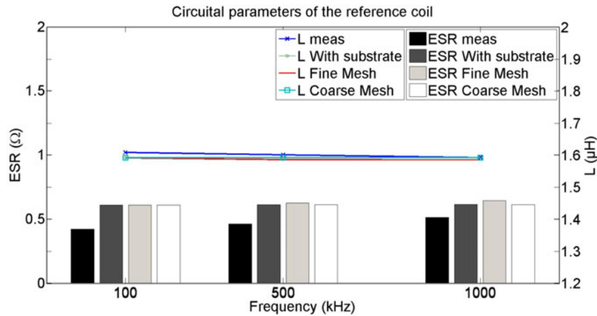
Fig. 6. Impact of the different modeling approaches for the reference coil: simulation results are compared with measurement ones.
