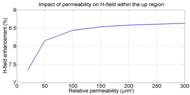
Fig. 29. H -field enhancement as function of the magnetic permeability of ferrite (other parameters frozen to their standard value).
