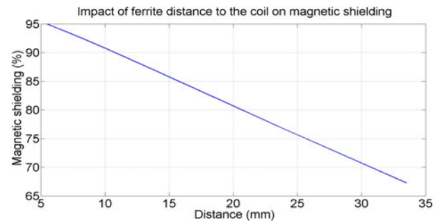
Fig. 22. Magnetic shielding as function of the distance between coil and ferrite (other parameters frozen to their standard value).
