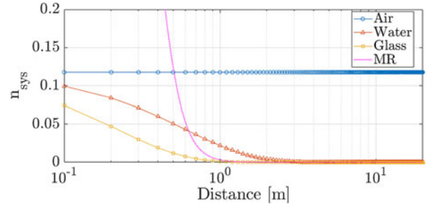
Fig. 8. Laser transmission efficiency through the air, pure water, and glass.
