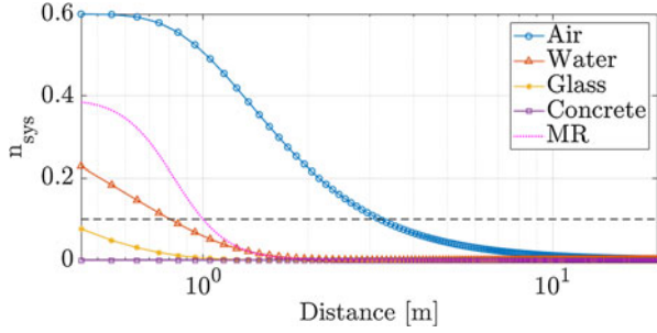
Fig. 7. Microwave transmission efficiency through the air, fresh water, glass, and concrete.
