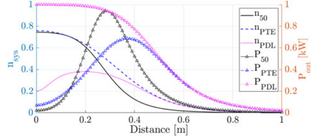
Fig. 6. Magnetic resonance using three coils with a fixed load, optimal PTE, and optimal PDL.
