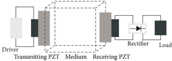
Fig. 3. Basic methodology of AET technology [39].
