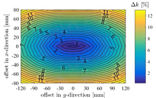
Fig. 8. Improvement of coupling coefficient \Delta k for tri-axial rotation.
