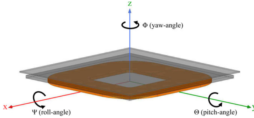
Fig. 5. Three angles of rotation in relation to the secondary coil.
