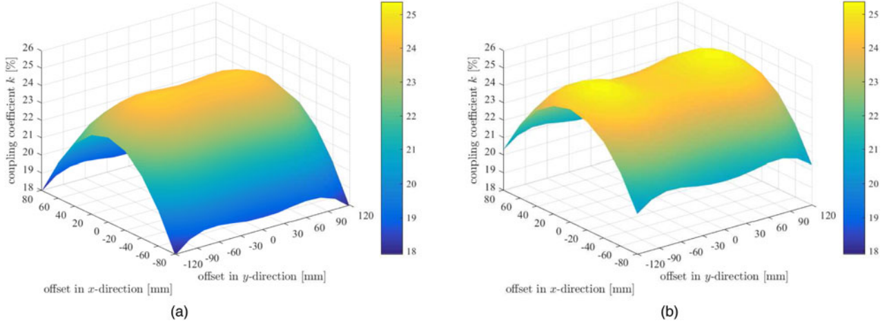
Fig. 9. Comparison of absolute values of coupling coefficient k . (a) Without rotation. (b) With bi-axial rotation.
