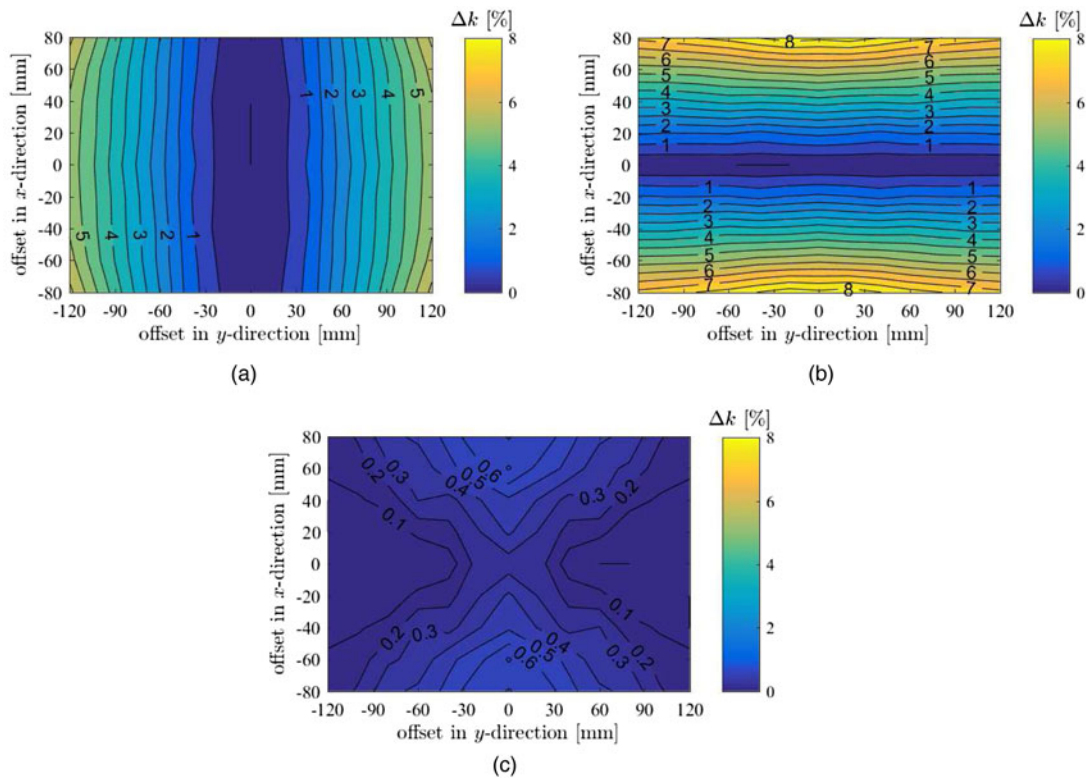
Fig. 6. Improvement of coupling coefficient \Delta k for mono-axial rotation. (a) Rotation in \Psi (around x -axis). (b) Rotation in \Theta (around y -axis). (c) Rotation in \Phi (around z -axis).
