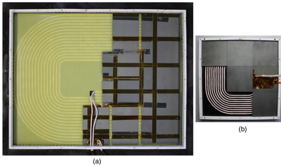
Fig. 4. Photograph of the measuring object. (a) Primary coil. (b) Secondary coil.
