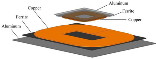
Fig. 3. Simulation model of the electromagnetic coupler.
