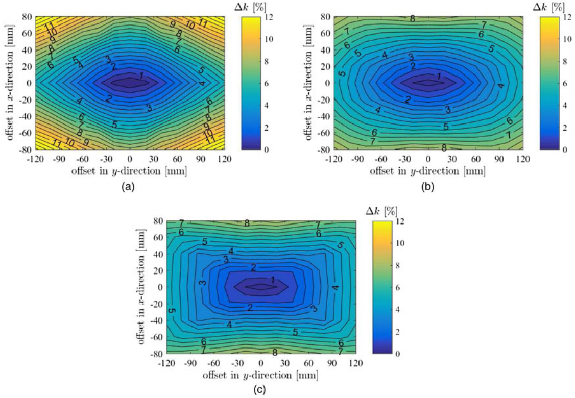
Fig. 7. Improvement of coupling coefficient \Delta k for bi-axial rotation. (a) Rotation in \Psi and \Theta (around x, y -axes). (b) Rotation in \Theta and \Phi (around y, z -axes). (c) Rotation in \Psi and \Phi (around x, z -axes).
