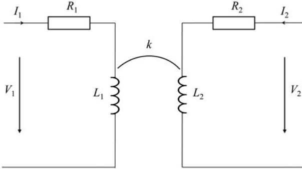
Fig. 2. Equivalent circuit of the electromagnetic coupler.
