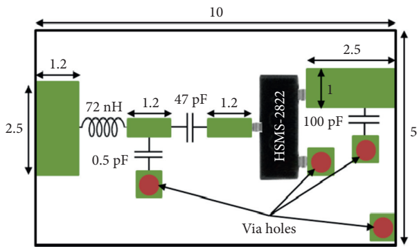
FIGURE 13: The geometry of the designed rectifier (all dimensions in mm).
